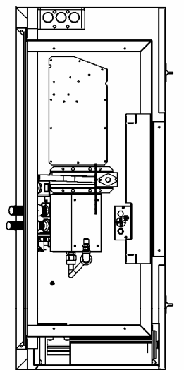
Mounting Tabs ZDV6000/3320 (Top View)
