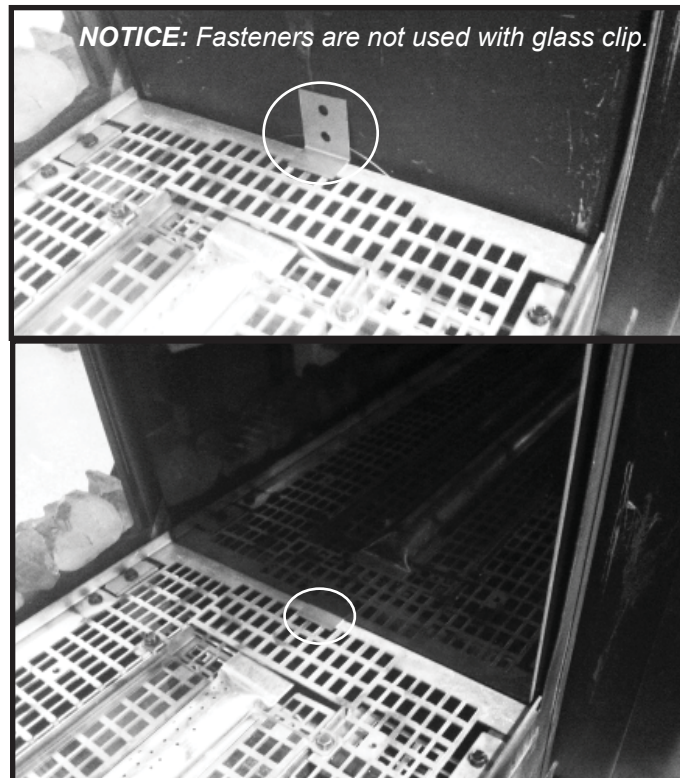
Figure 10.8 Position Glass Clip and Install Glass Panel
