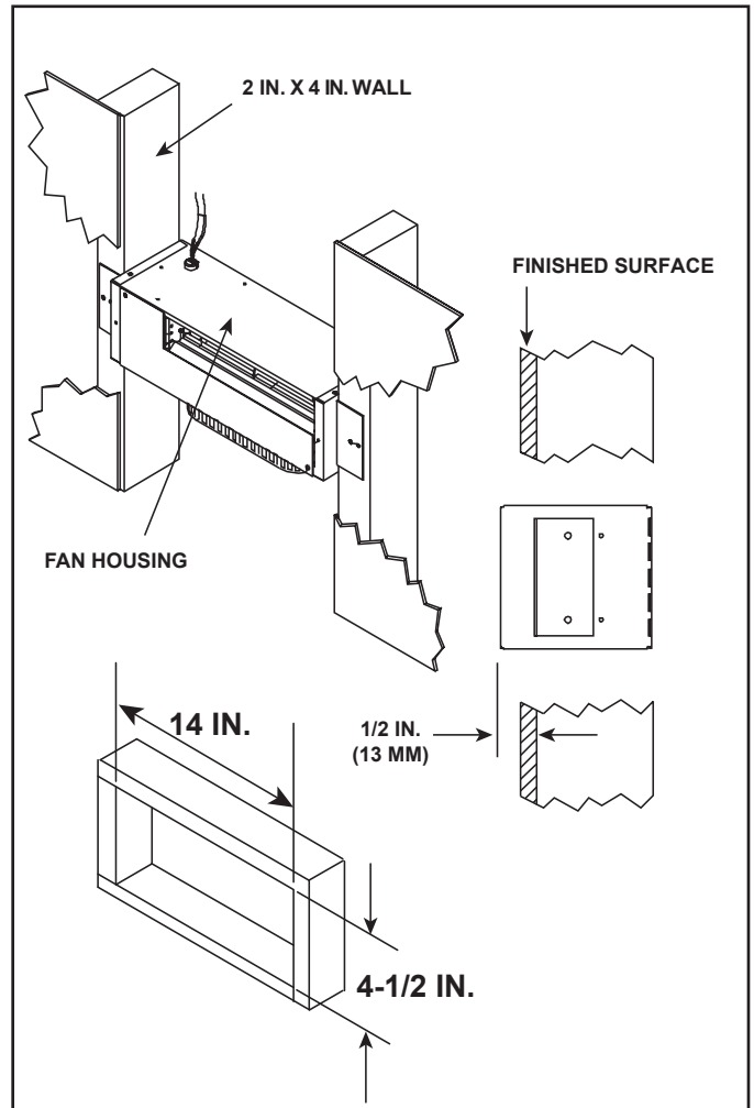
Figure 6.11 Wall Mounting (2 X 4) ←
