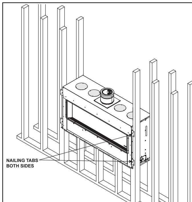
Figure 6.2 Nailing Tab Locations
