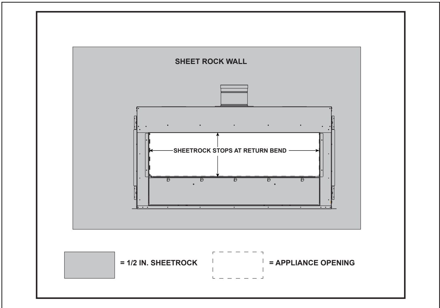
Figure 10.2 Sheetrock Detail for Both Finishing Methods
