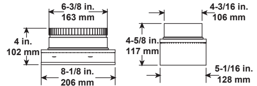
DVP-2SL Adapter (Included)
