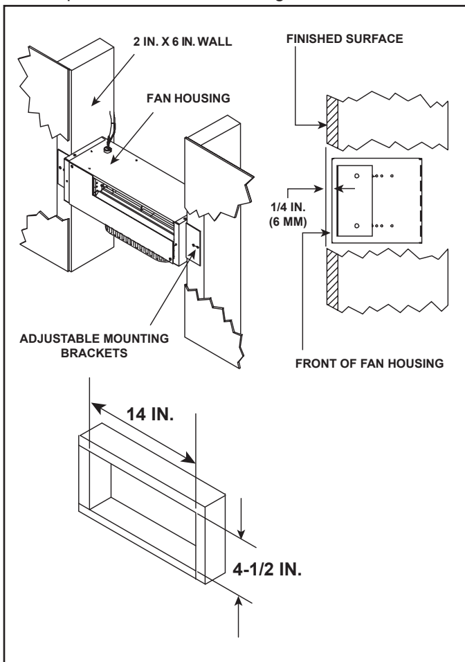
→ Figure 6.10 Wall Mounting (2 X 6)
