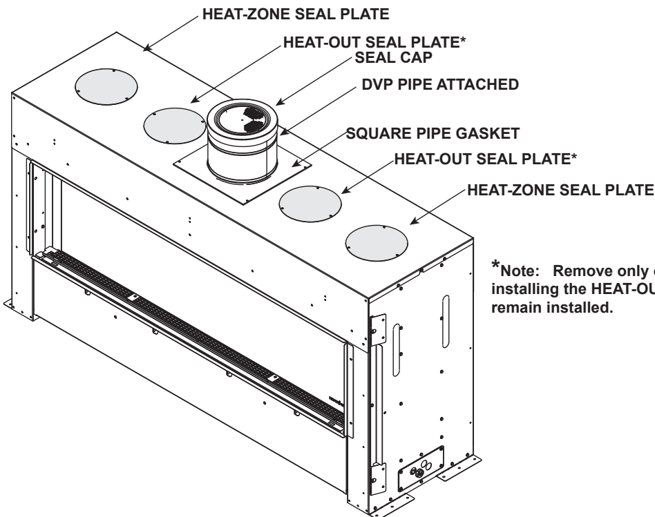
Figure 6.1 Vent Collar Preparation
