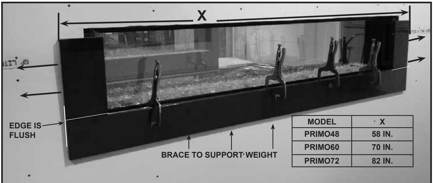
Figure 10.28. Apply Adhesive For Top and Bottom Granite
