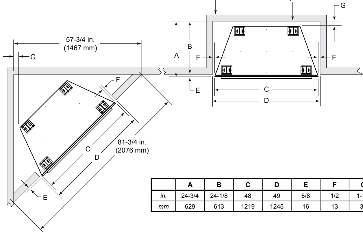
Figure 3.1 Appliance Locations
