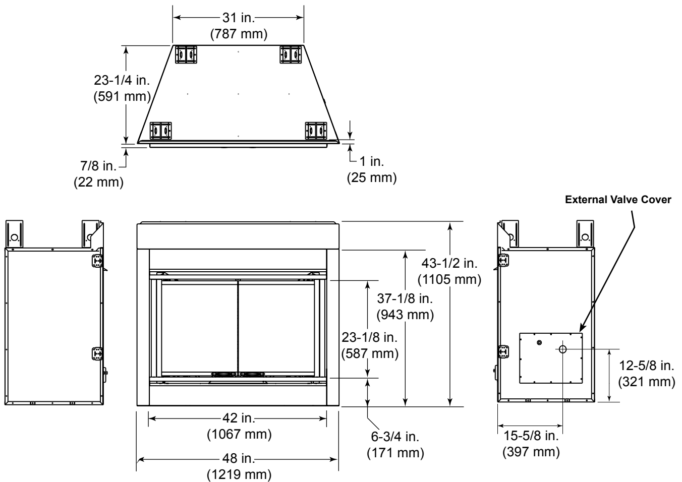
Figure 13.1 Appliance Dimensions
